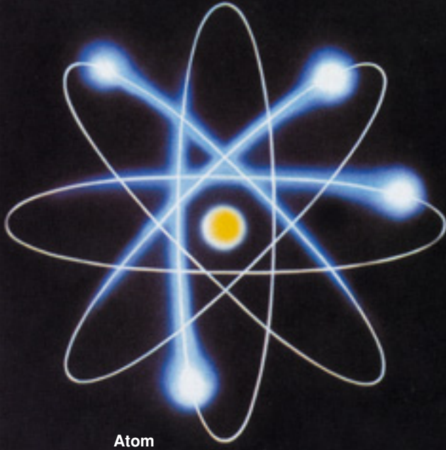
Atom
