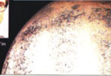
Spiral Galaxy M81 NASA Spitzer Space Telescope image of the spiral galaxy M81, located some 12 million light years from Earth. The infrared radiation emitted by Polycyclic Aromatic Hydrocarbons (PAHs) molecules is shown in red.
