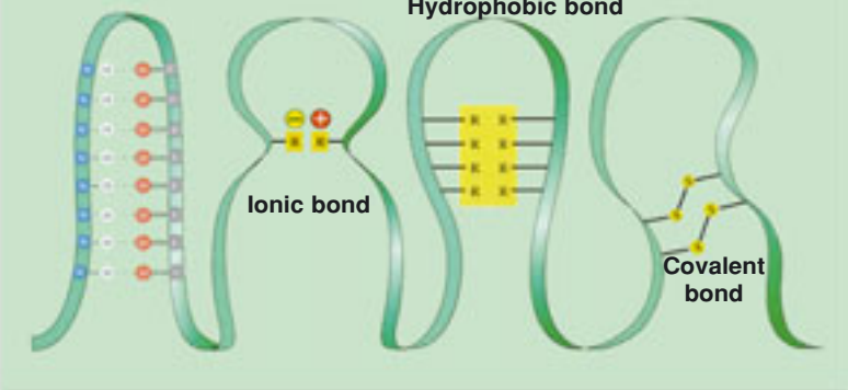
Hydrogen bond
