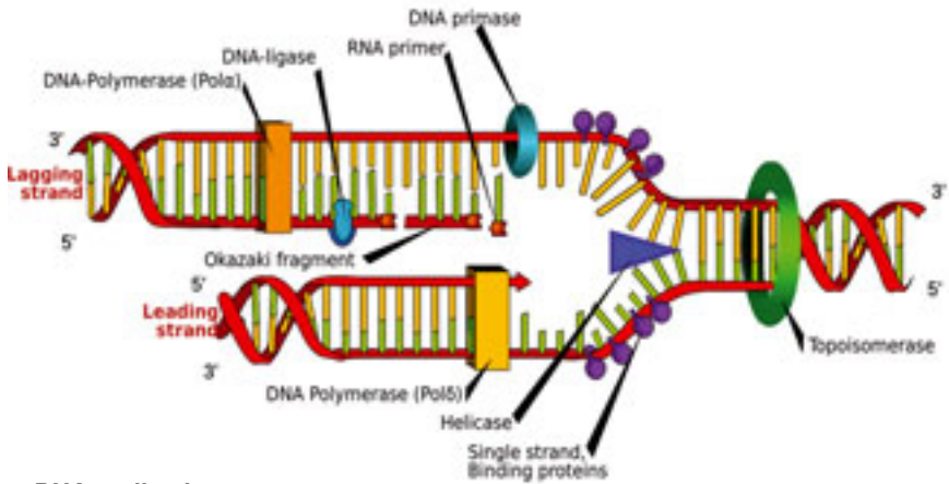
DNA replication
